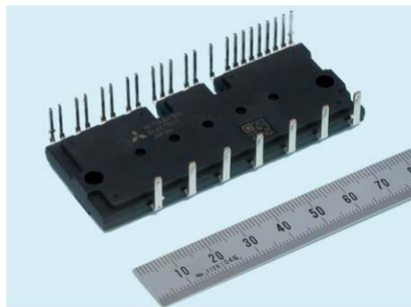
Large hybrid SiC DIIPM (PSH50YA2A6)
